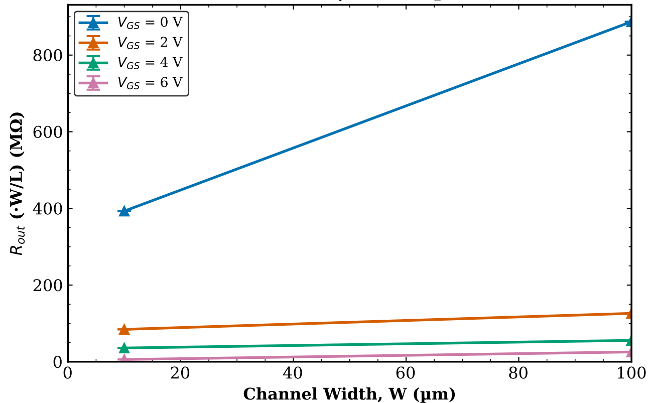
TFT3 Transistor 2 R_{out} vs W | L = 80\text{ }\mu\text{m}
